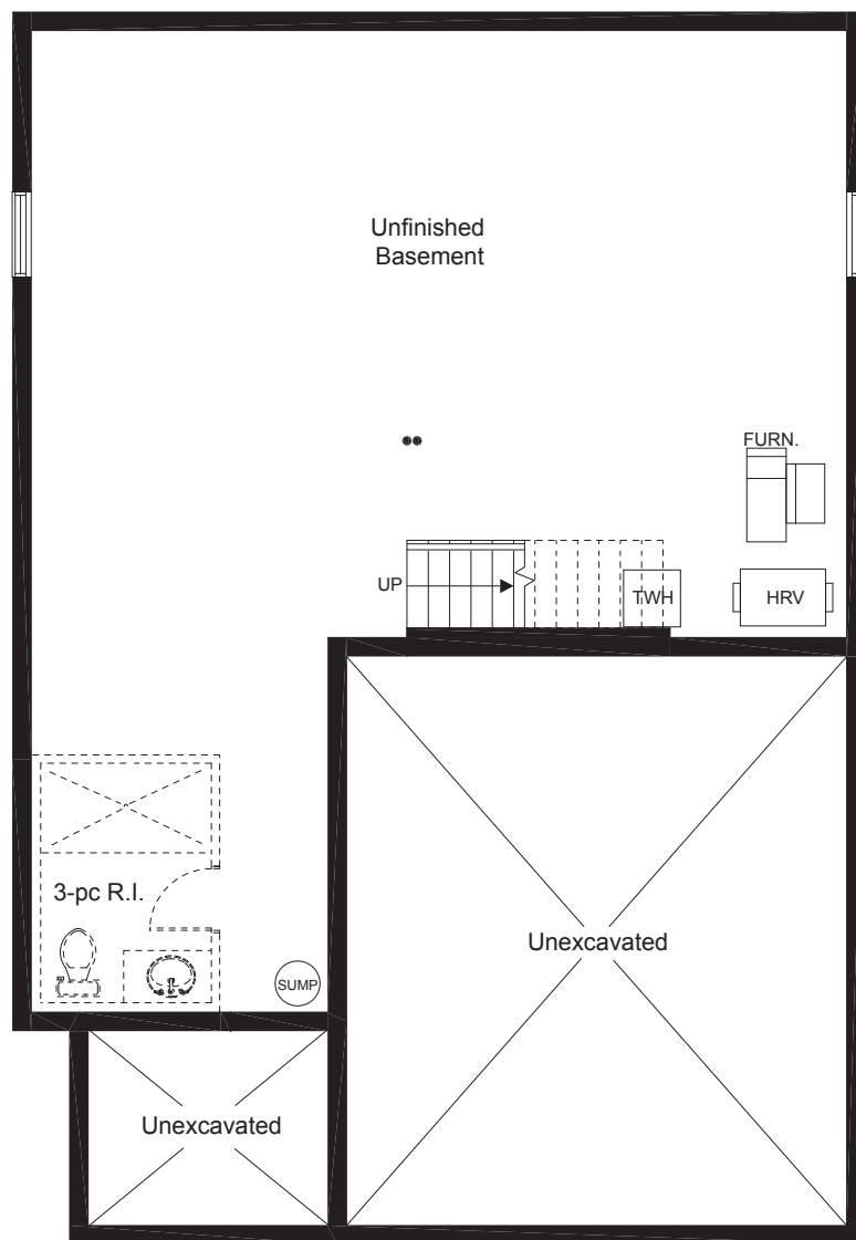
BASEMENT
