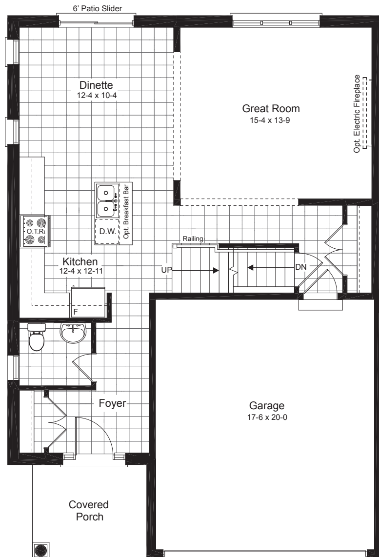
MAIN FLOOR
